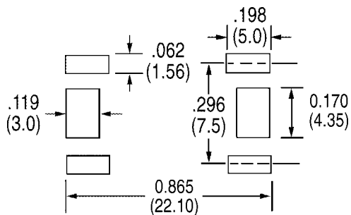
SOLDER PAD LAYOUT
