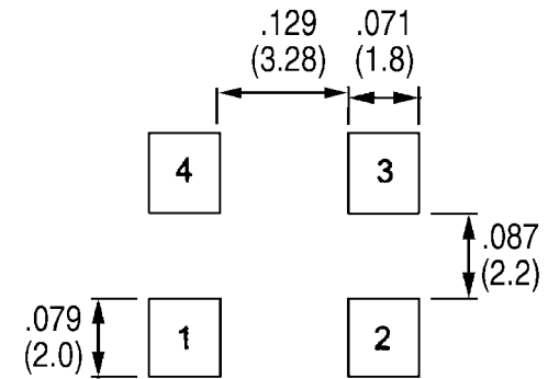
SOLDER PATTERN LAYOUT
